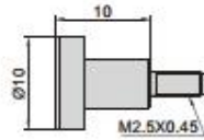
Flat Point
