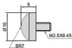
Spherical Point
